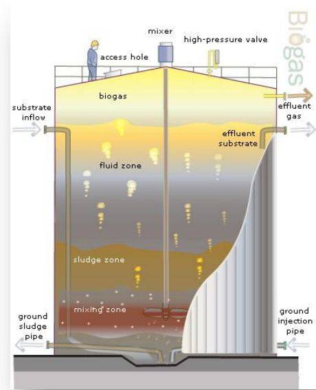
Figure 1. Cross section of typical anaerobic digestion plant.
